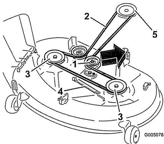
Figure 54 Mower Decks with 2 Blades
