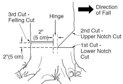
Figure 14 - Felling A Tree
