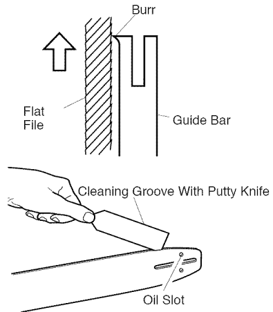
Figure 21 - Guide Bar Maintenance
