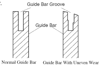
Figure 20 - Guide Bar Cross Section Showing Uneven Bar Wear
