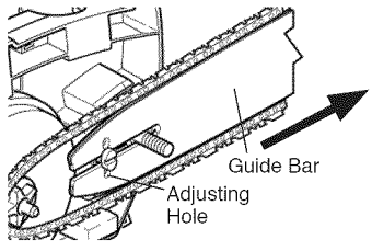
Figure 6 - Pulling Guide Bar
