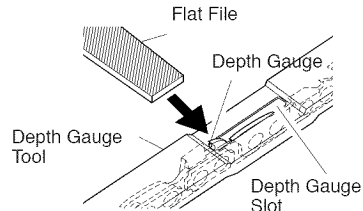
Figure 24 - Depth Gauge Tool On Chain
