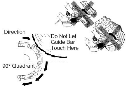
Figure 1 - Kickback Hazard Example: Do Not Let Nose of Guide Bar Touch Object While Chain is Moving
