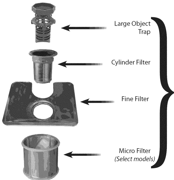
FILTER SYSTEM
